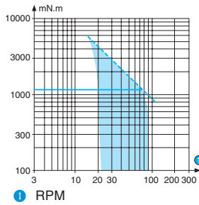
Nominal speed and torque curves 82 802 0
