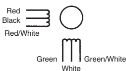
B - Connections in parallel
