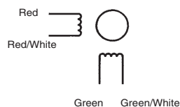
A - Connections in series
