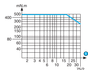
Torque/speed curves 82 524 4
