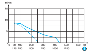
Nominal value dynamic curves 4 phases - 115 Ω
