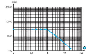
Torque / speed curves 80 513 5
