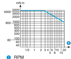
Torque/speed curves 80 547 0
