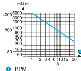
Torque/speed curves 80 527 4
