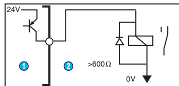
Examples of encoder output, direction, torque limit cabling (brown - red - violet)
