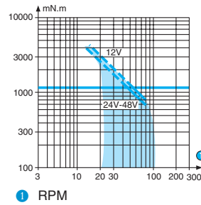
Nominal speed and torque curves 82 812 0
