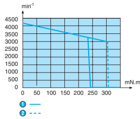
Speed/torque
