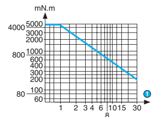
Torque/speed curves 80 527 0
