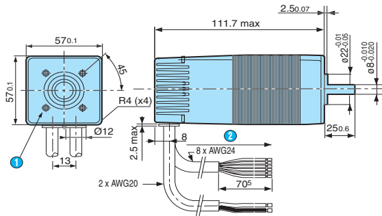
Short version 80 180 0
