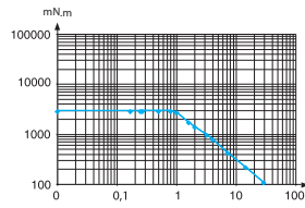
Graph of torque versus speed 82 333 5
