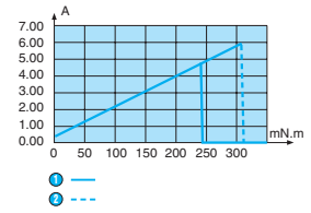
Current/torque
