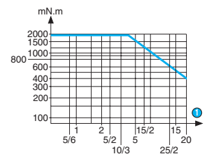
Torque/speed curves 82 529 4
