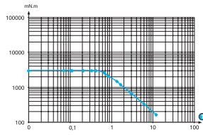
Torque / speed curves 80 513 0
