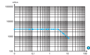
Torque / speed curves 80 533 0
