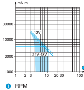
Nominal speed and torque curves 82 812 5
