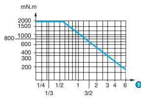
Graph of torque versus speed 82 304 0
