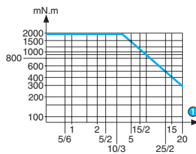
Torque/speed curves 82 529 0
