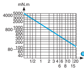
Torque/speed curves 80 517 0
