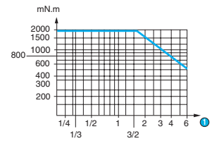
Graph of torque versus speed 82 305 0
