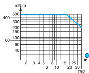
Torque/speed curves 82 524 0
