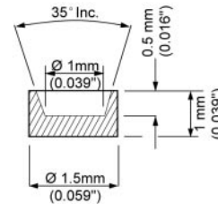
SMOX/060/TP Contact Test Point
