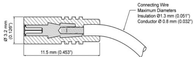
LS/B1/093 (All 1 mm (0.040") Snaplox)
