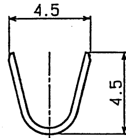
B-B SEC.
