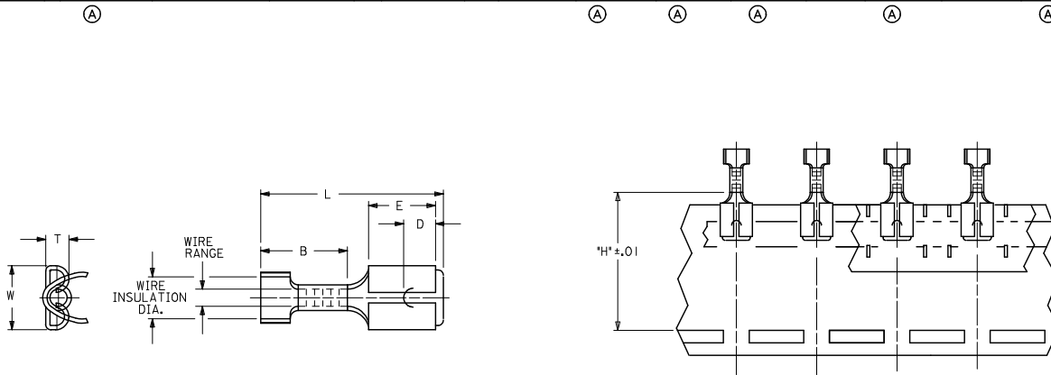
Ⓐ TAPE-MOUNTED PARTS
