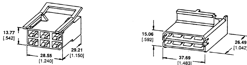
6 Position (mates with Tab Housing) Part No. 180906
