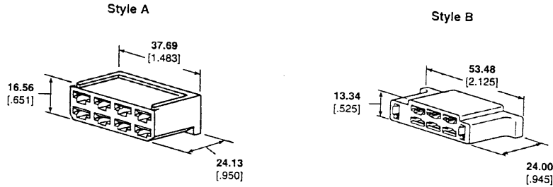
Receptacle Housings
