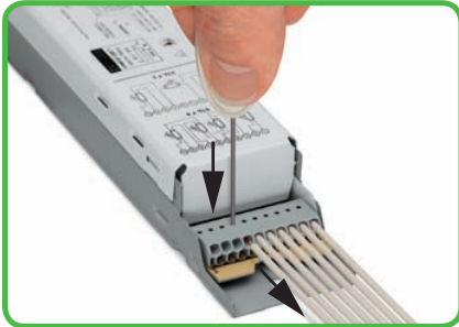
Conductor removal using a disconnecting tool Ø 1.2 mm/0.047 in
