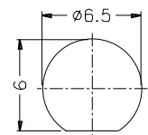
RECOMMENDED MOUNTING HOLE (建議架設孔)
