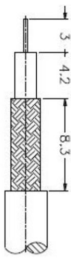
RECOMMENDED CABLE STRIPPING DIM'S
