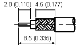
Stripping Dimension
