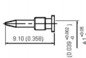
Stripping Dimension Dimensions : Millimetres (Inches)
