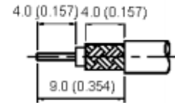
Stripping Dimension Dimensions : Millimetres (Inches)
