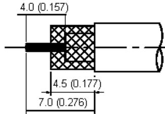
Stripping Dimension
