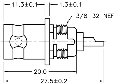
BODY
