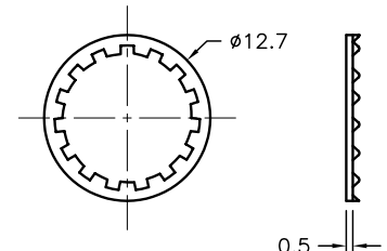
LOCK WASHER
