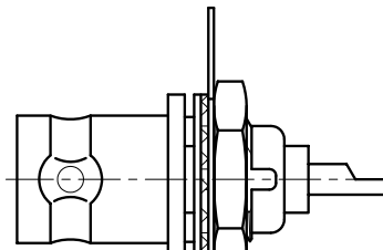
ASSEMBLY
