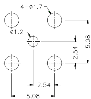
PCB MOUNTING HOLE
