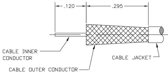
CABLE PREPARATION SCALE: NTS
