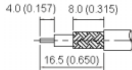
Stripping Dimension Dimensions : Millimetres (Inches)
