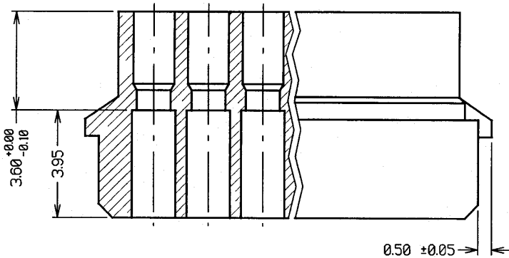
PART SECTION P-P
