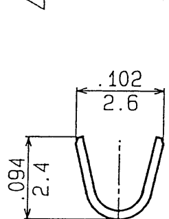
WIRE BARREL
