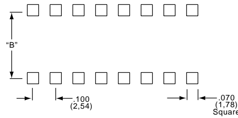
Recommended Pad Pattern Tolerance ± .002 (0,05)
