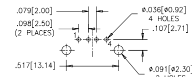
RECOMMENDED P.C.B. LAYOUT (COMPONENT SIDE OF BOARD)
