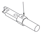
PART NUMBER 356-157-4 TERMINATING BLADE 157 SERIES CONNECTORS PLUG AND RECEPTACLE
