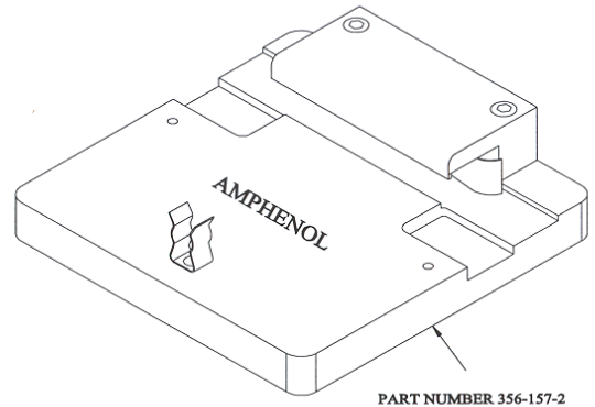
PART NUMBER 356-157-2 HOLDING FIXTURE FOR 157 SERIES CONNECTORS PLUG AND RECEPTACLE
