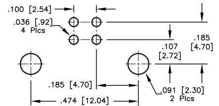
SUGGESTED MOUNTING CONFIGURATION
