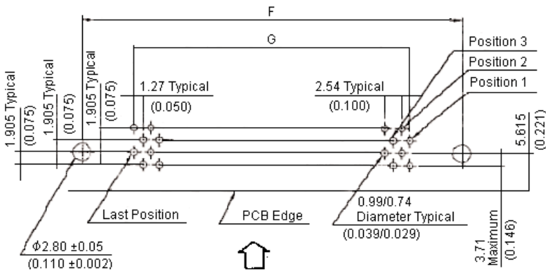
Connector Mating Side Recommended PCB Hole Pattern
