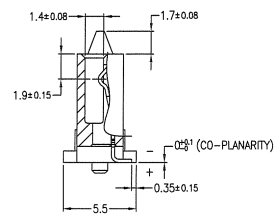
SECT-Y-Y
