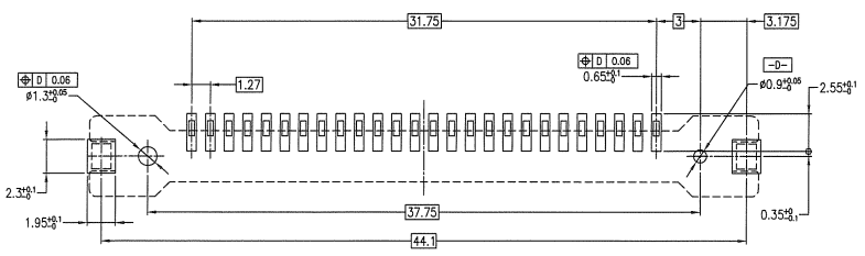
RECOMMENDED MOUNTING LAYOUT TOLERANCE UNLESS OTHERWISE ±0.1
