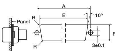
Rear Panel Mounting
