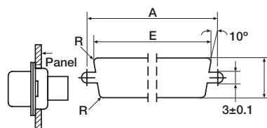
Front Panel Mounting
