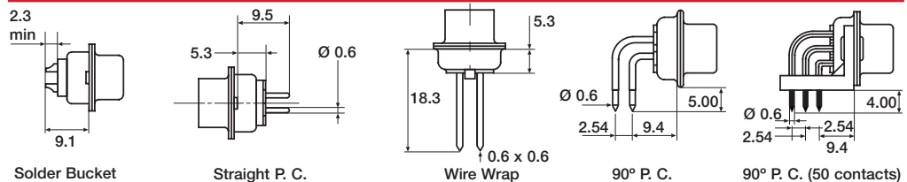
Solder Bucket
