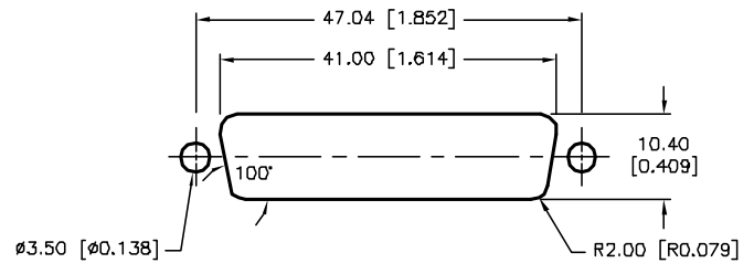
PANEL CUTOUT
