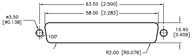
PANEL CUTOUT
