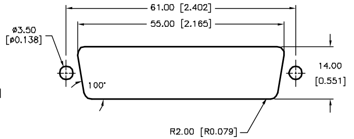
PANEL CUTOUT
