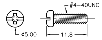
Screw (2pcs)
