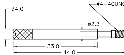
THUMB SCREW
