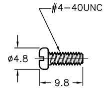
SCREW
