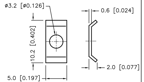
SADDLE WASHER (2pcs)
