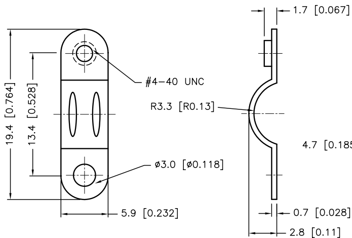
CABLE CLAMP (2pcs)
