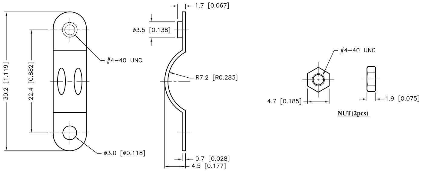
CABLE CLAMP (2pcs)
