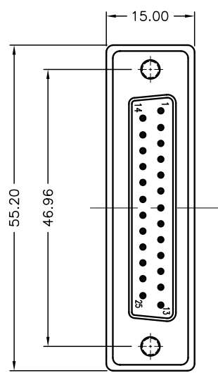
DB-25 Pin Male
