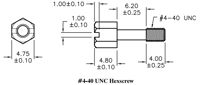
#4-40 UNC Hexscrew
