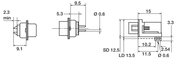
Solder Bucket
