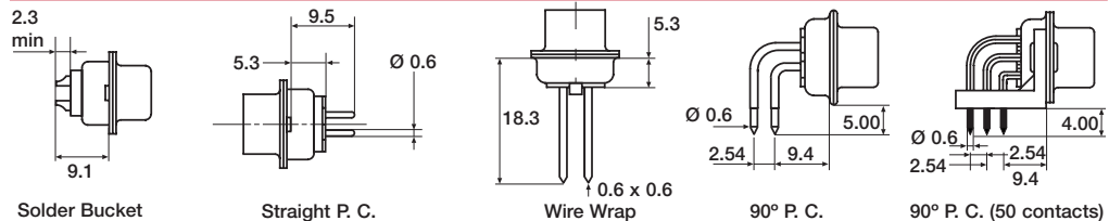
Solder Bucket
