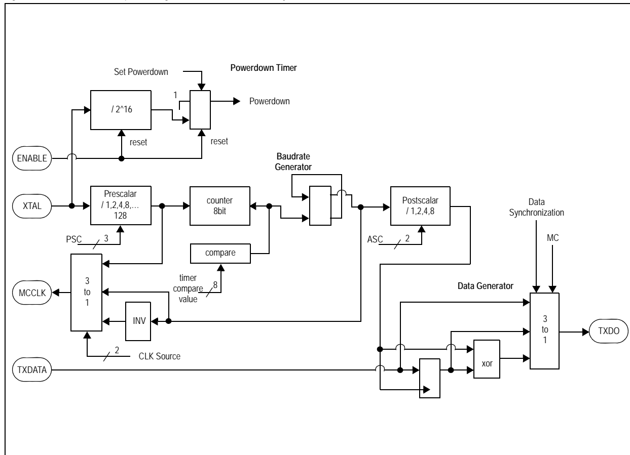
Figure 5. Functional Description Diagram of Timers and Data Synchronization
