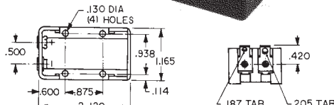
CAT. NO. 1295 Quick-Fit/Solder Lug Terminals
