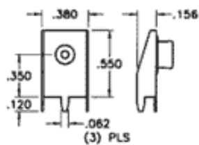
Mounting Detail
