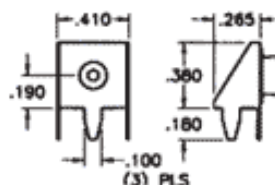
Mounting Detail
