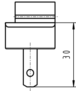
USA-Stecker 1717715 USA-plug 1717715
