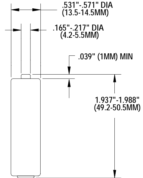
Dimensions shown are ANSI / IEC standards
