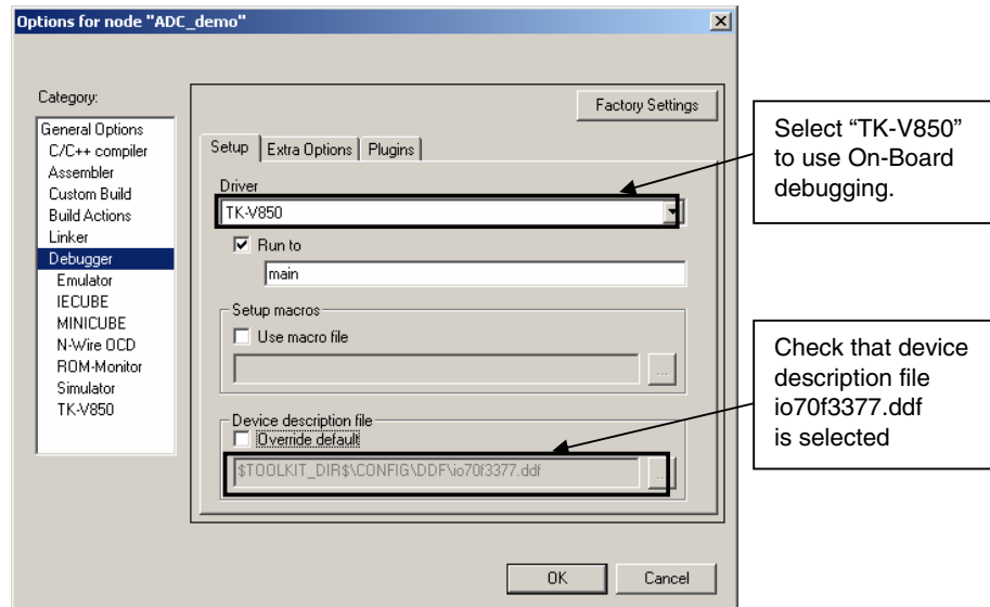
Figure 64: IAR debugger options 1/2
