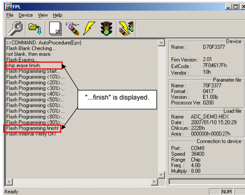
Figure 61: After EPV Execution
