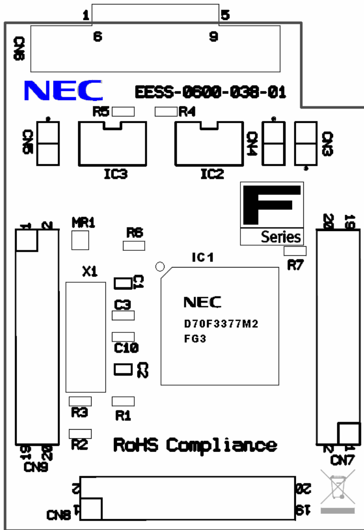
Figure 4: V850ES/Fx3 – CAN it! CPU module components
