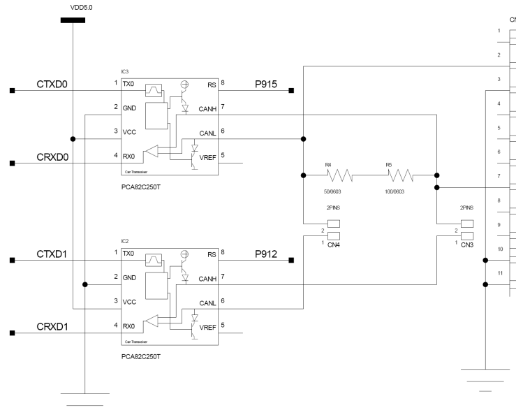
Figure 5: CAN transceivers
