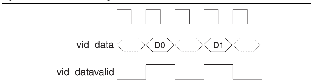
Figure 5-5. vid_datavalid Timing
