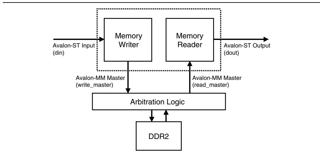
Figure 5-24. Frame Buffer Block Diagram
