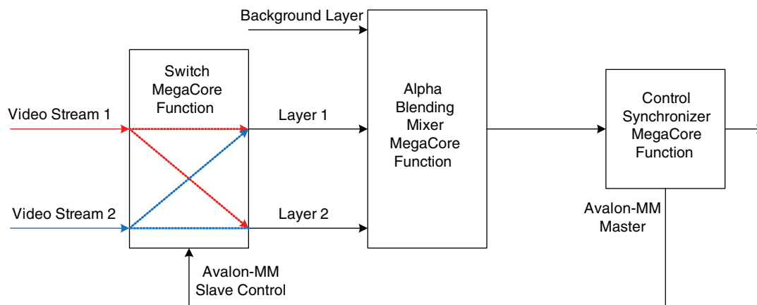
Figure 5–28. Example of a layer Switching System
