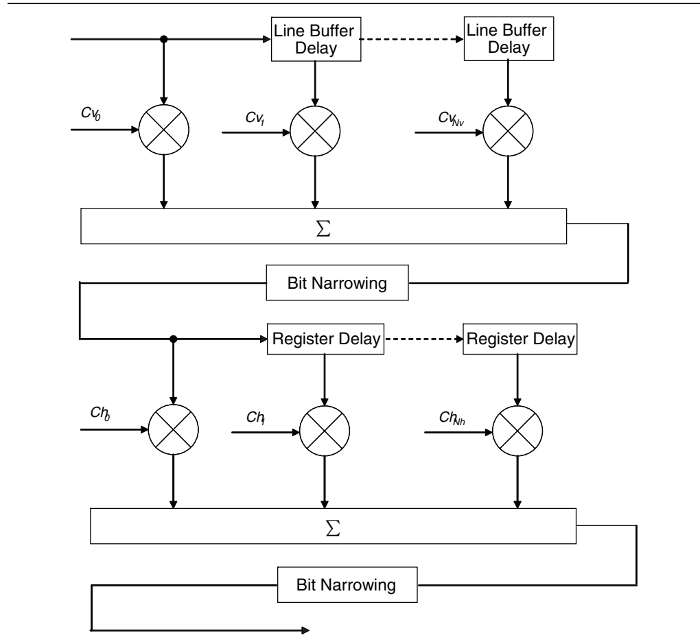
Figure 5-26. Polyphase Mode Scaler Block Diagram
