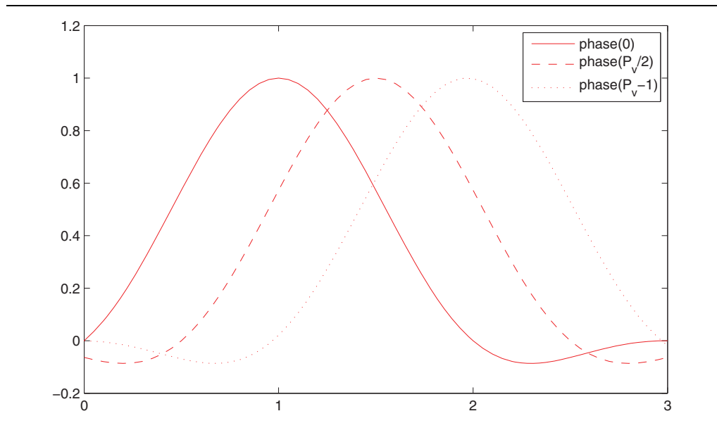
Figure 5-27. Lanczos 2 Function at Various Phases
