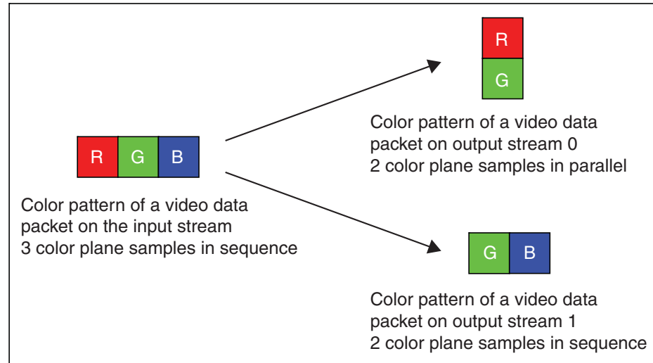
Figure 5-16. Example of Splitting and Duplicating Color Patterns
