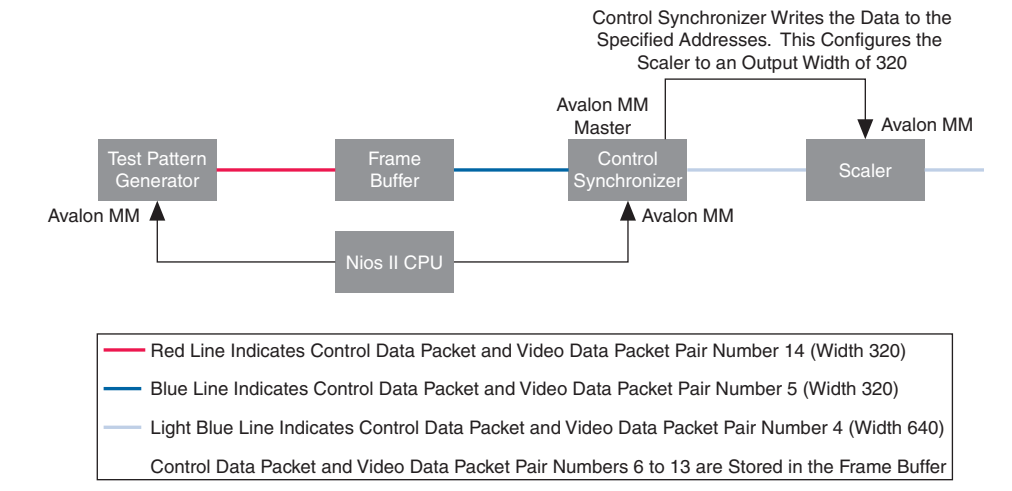
Figure 5-19. Test Pattern Generator Change
