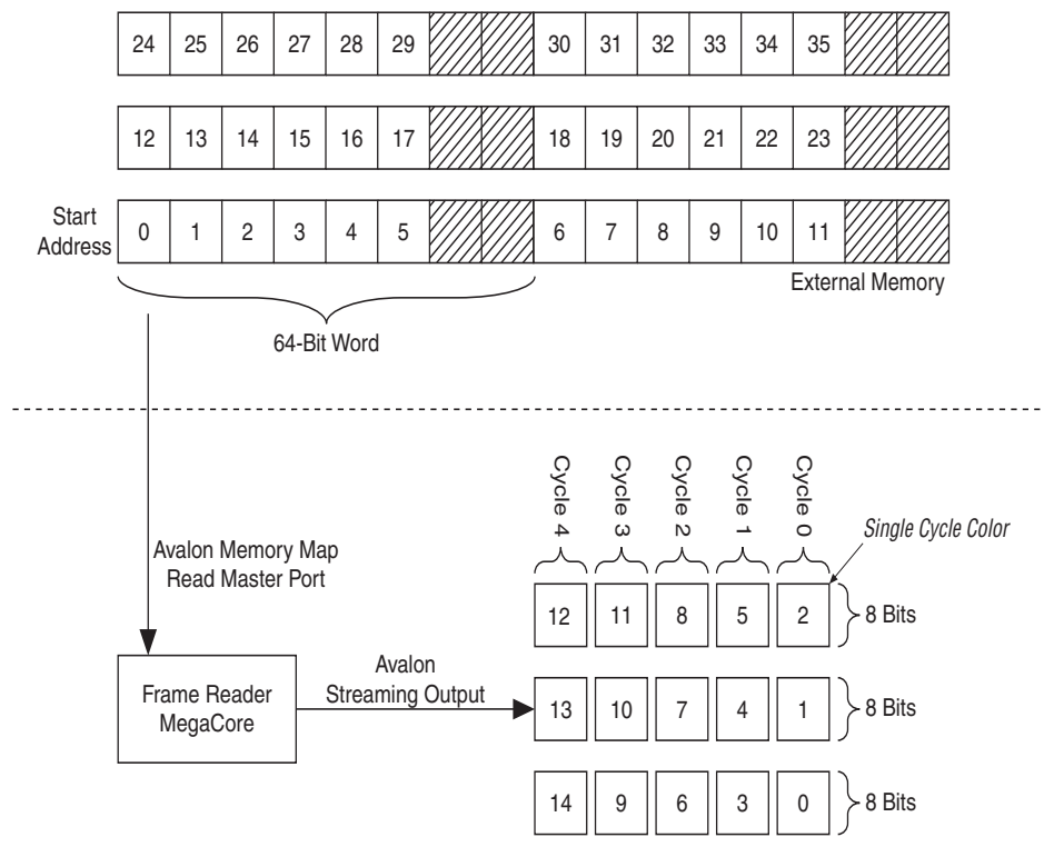
Figure 5-25. Frame Reader Output Pattern and Memory Organization
