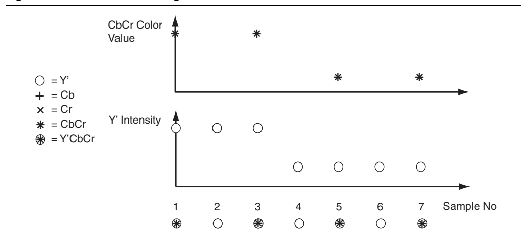
Figure 5-2. 4:2:2 Data at an Edge Transition
