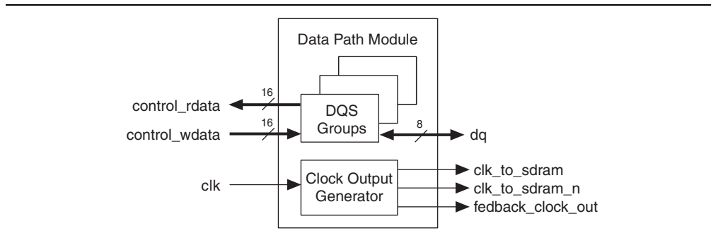
Figure 3-2. Datapath
