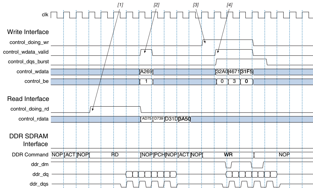
Figure 3-3. Datapath Timing
