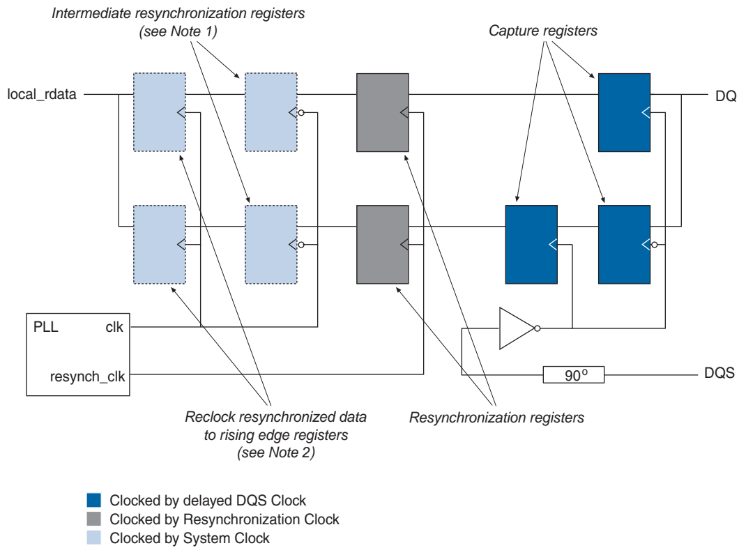
Figure A-1. Resynchronization Registers
