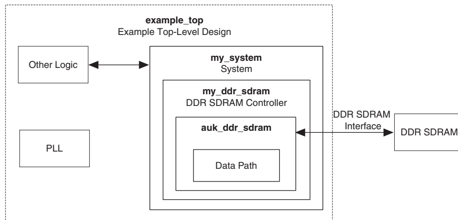
Figure 2-1. System Naming
