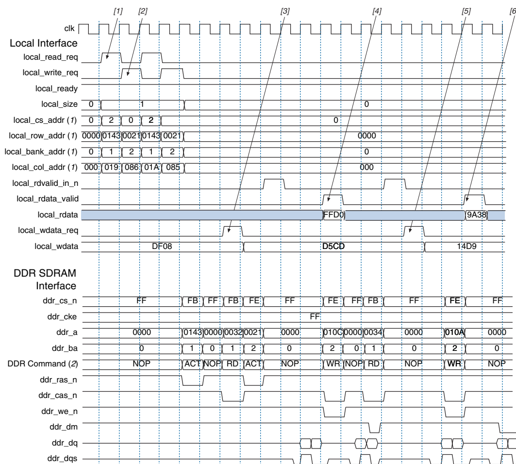
Figure 3-15. Read-Write-Read-Write
