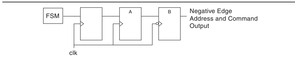
Figure 3–21. Additional Pipeline Registers—A = On, B = Off, C= On
