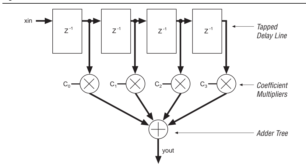
Figure 1-1. Basic FIR Filter
