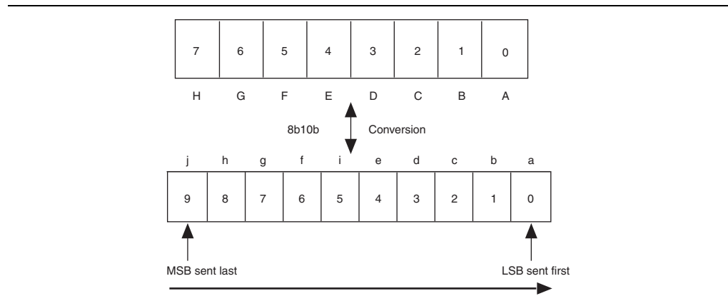
Figure 3–1. 8b10b Conversion
