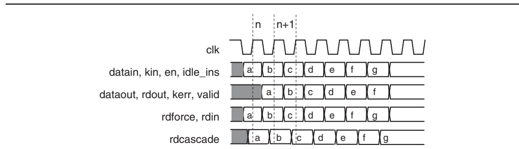
Figure 3-6. Encoder Timing Diagram—One Cycle Latency
