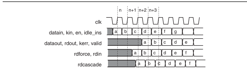
Figure 3-5. Encoder Timing Diagram—Three Cycle Latency
