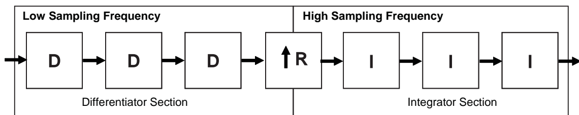
Figure 4-4. Three Stage Interpolation Filter
