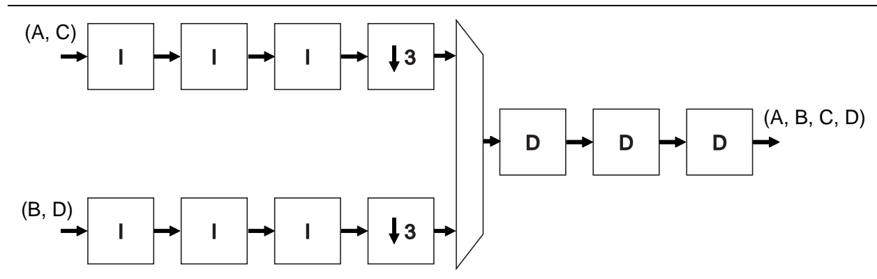
Figure 4-6. Multiple Input Single Output Architecture
