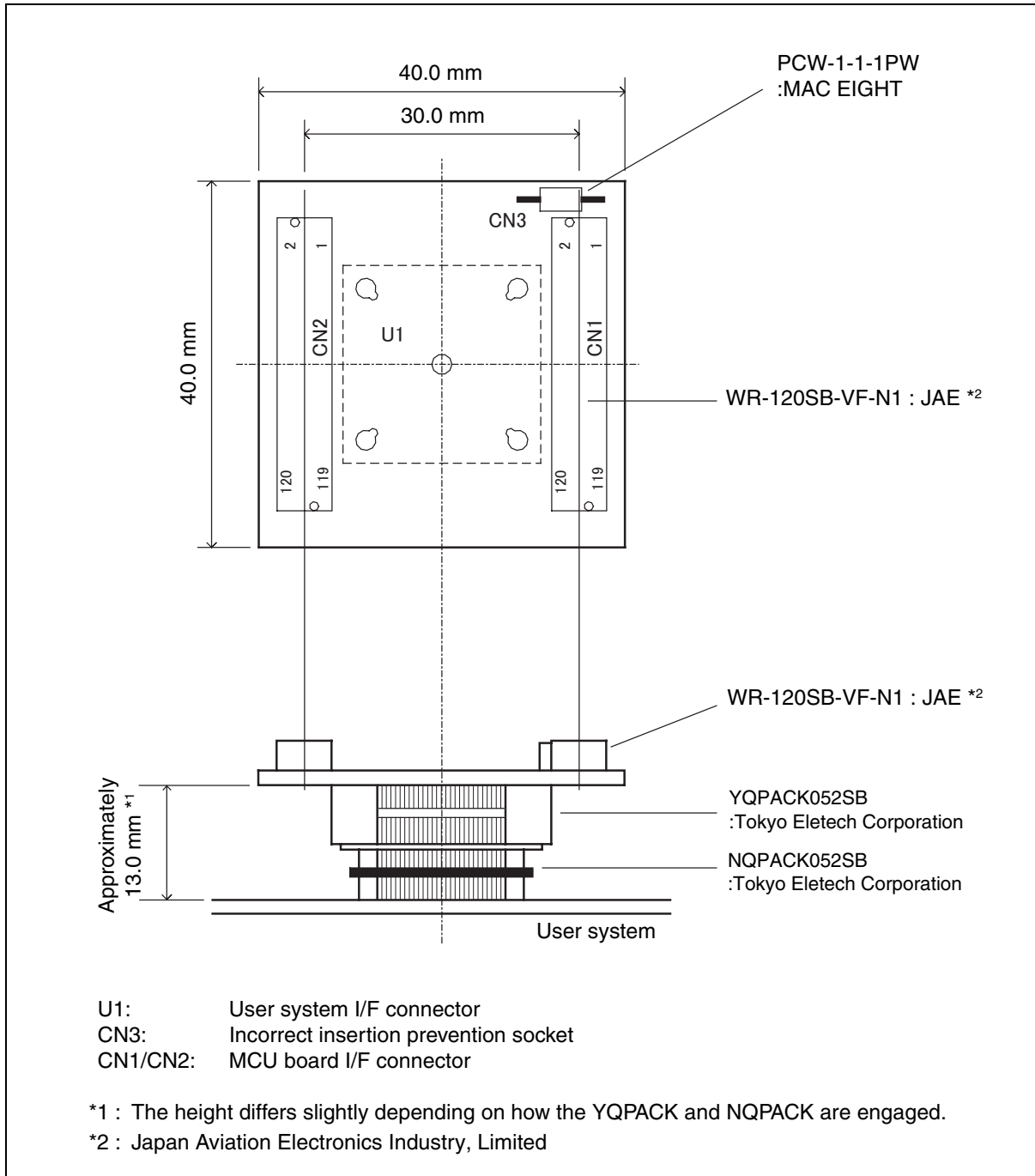
Figure 2 Header Board Dimensions
