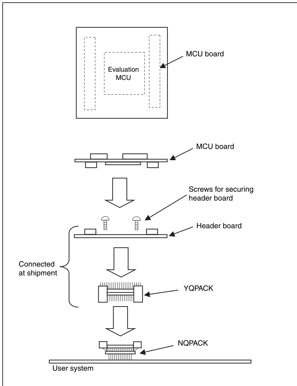
Figure 5 Connecting MCU Board/Header Board to User System
