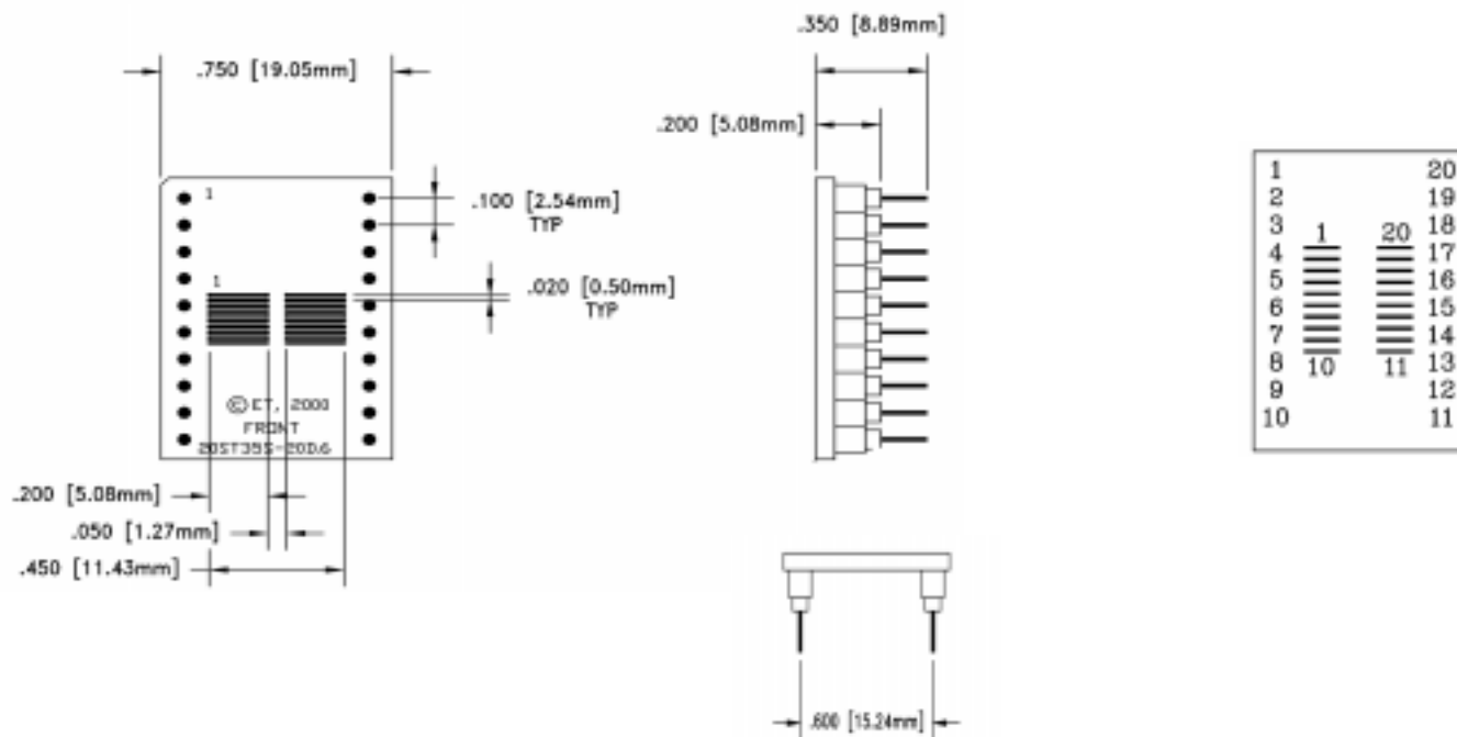
Top View
