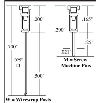
Bottom Male Pin Types
