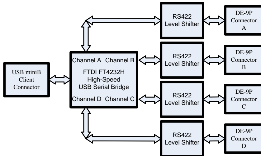
Figure 1.2 USB-COM422-PLUS4 Block Diagram
