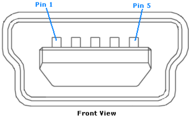
Figure 4 USB Mini-B type connector and pin assignments.
