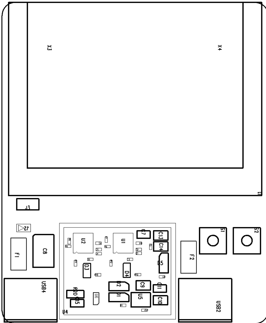
Figure 5 Assembly TOP
